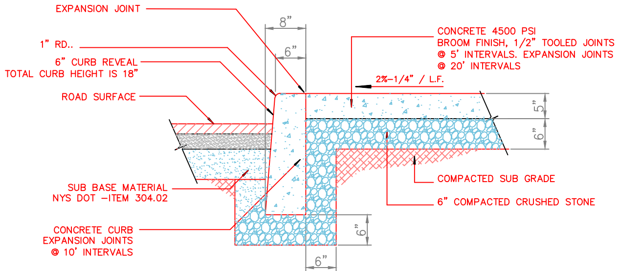
CONCRETE SIDEWALK AND STANDARD CURB DETAIL
