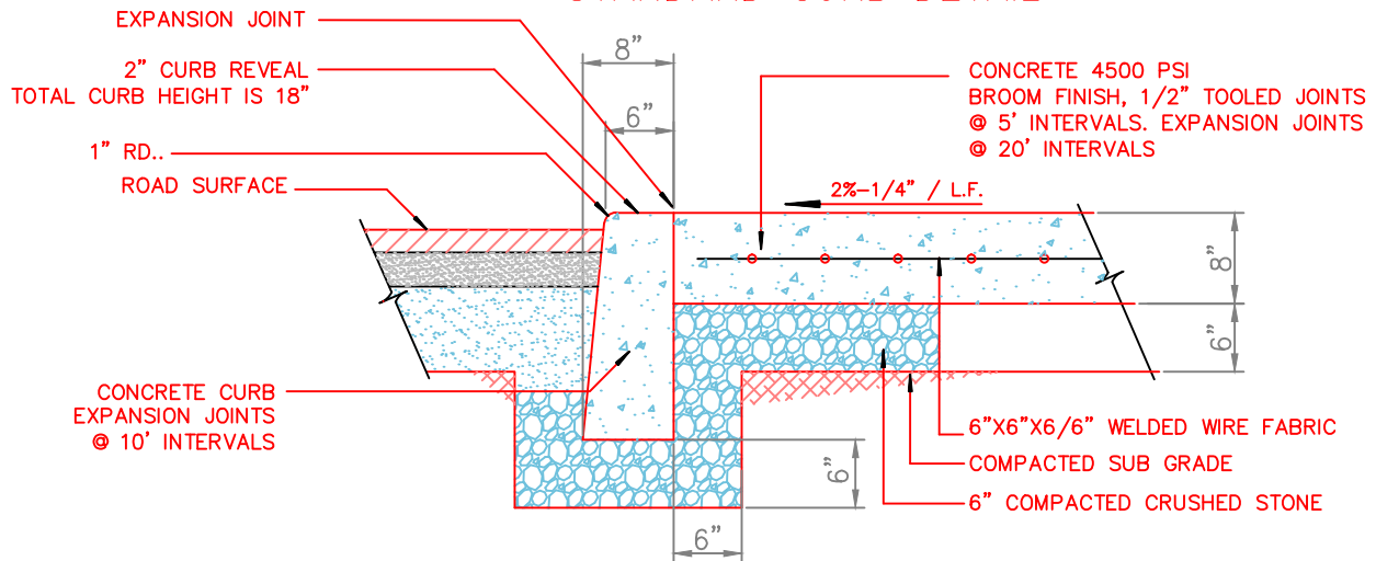
CONCRETE DRIVEWAY AND DROP CURB DETAIL
